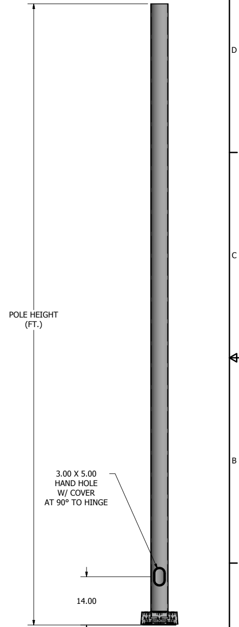
POLE DETAIL
